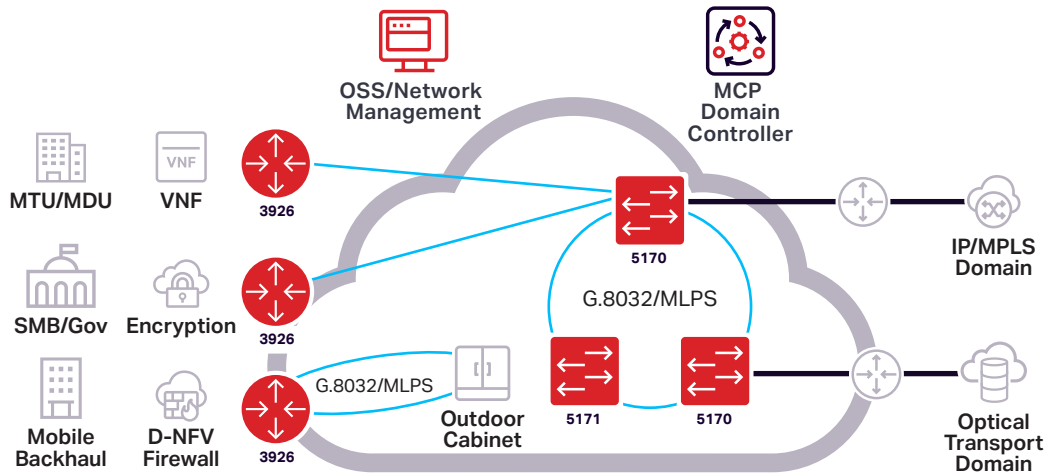
Figure 5. Typical D-NFV deployment with 3926 as smart CPE
